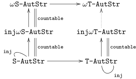
Figure 2: Relationship of classes of automatic structures
