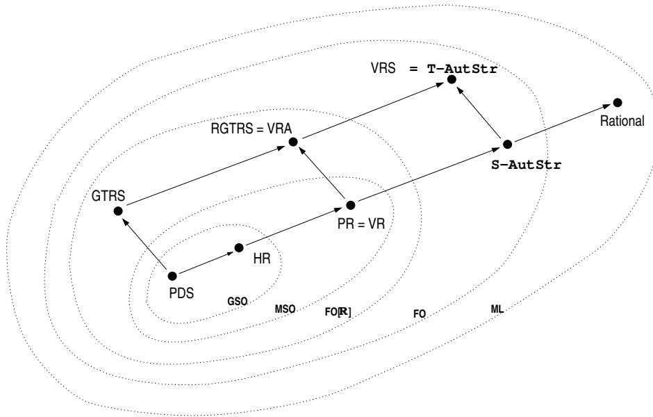
Figure 1: Relationship of graph classes and logical decidability boundaries.
